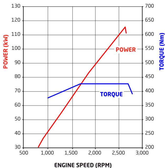
Isuzu 4HK1-TCN
