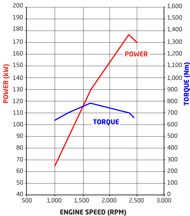
Isuzu N-4HK1-TCH
