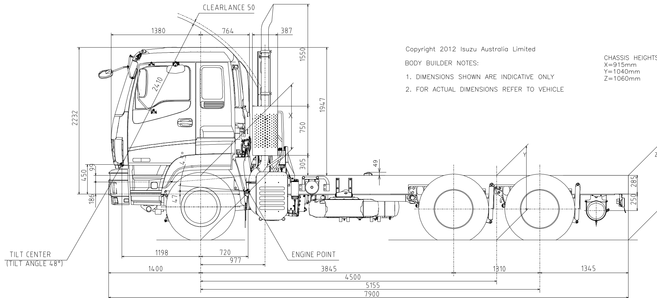
CH 2011MY Isuzu Giga CXY 455 medium premium
